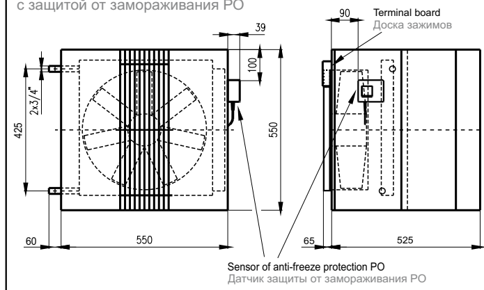
Fig. 3 VCP-03-055 module - warm water / hot water with PO
