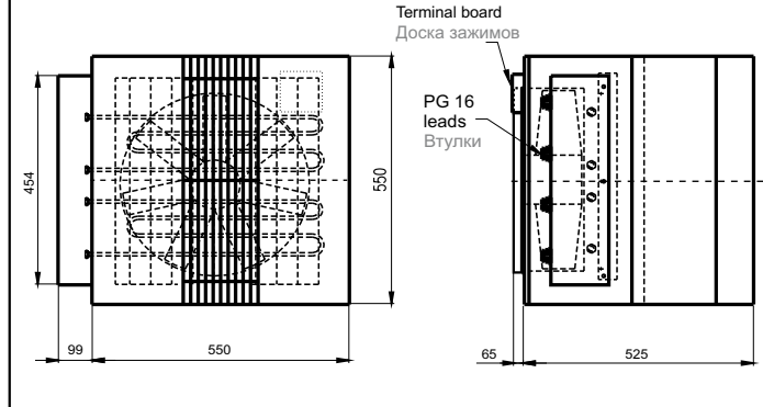
Fig. 3 VCP-03-055 module - warm water / hot water with PO
