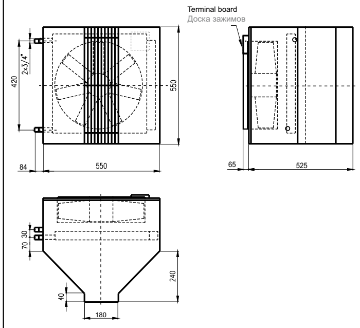
Fig. 1 VCP-03-055 module - warm water / hot water
